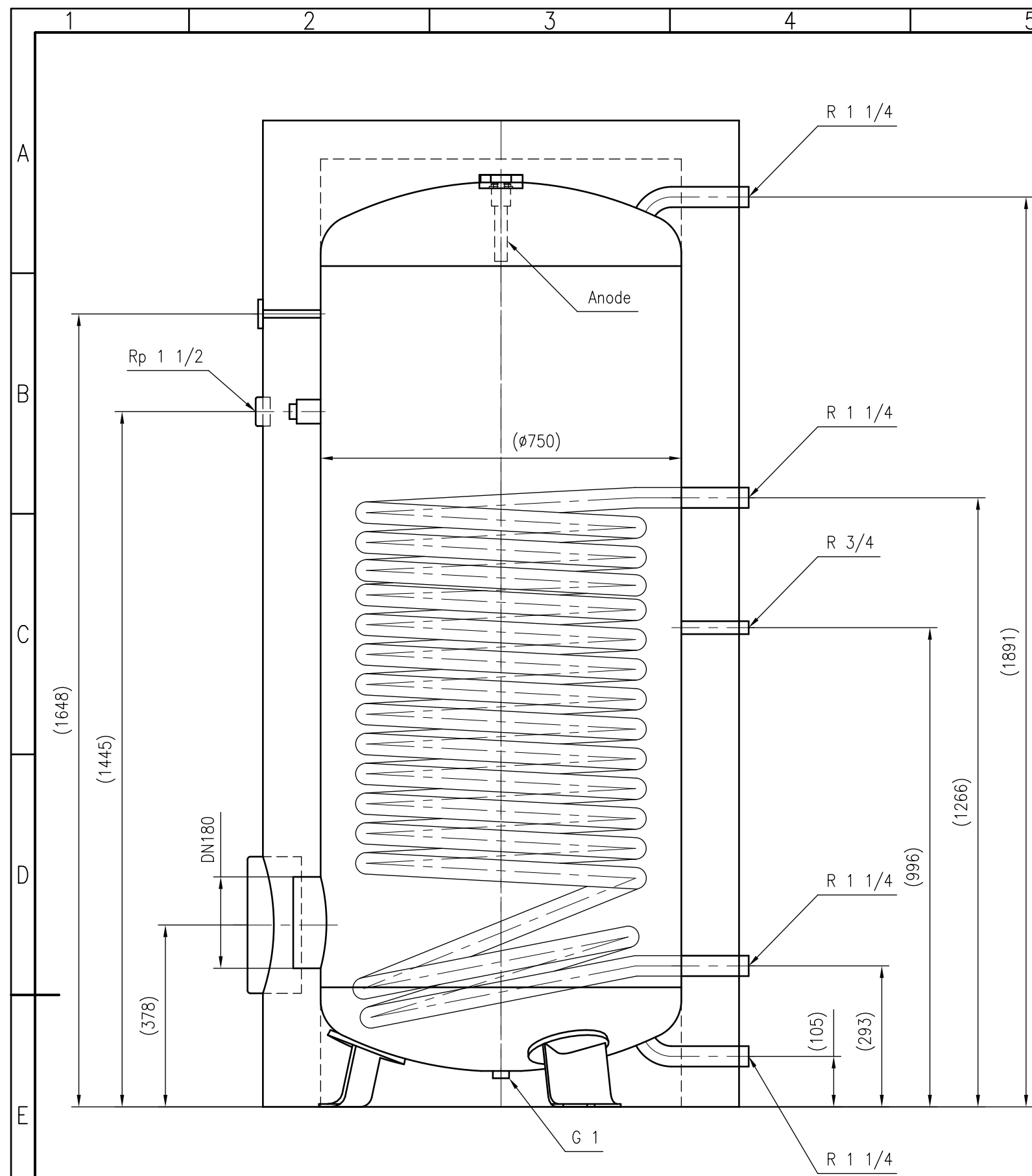
Side view
